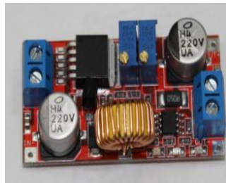
XL4015 MODULE WITH POT I/P:- 5V- 38V O/P:- 1.25V- 32V / 5A
