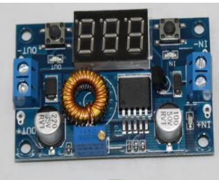
XL4015 LED MODULE I/P:- 4V- 38V O/P:- 1.25V-36V / 5A
