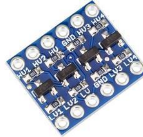
Logic Level Bi-Directional 4 Channel Converter Module
