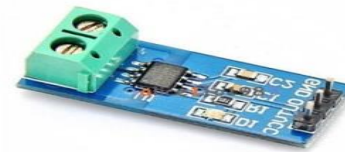
Current Sensor ACS712 30AMPS/ 5AMPS / 20AMPS
