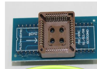
PLCC44 TO DIP 40 Adapter
